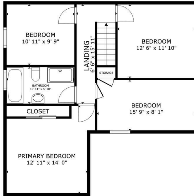
FLOOR 2
